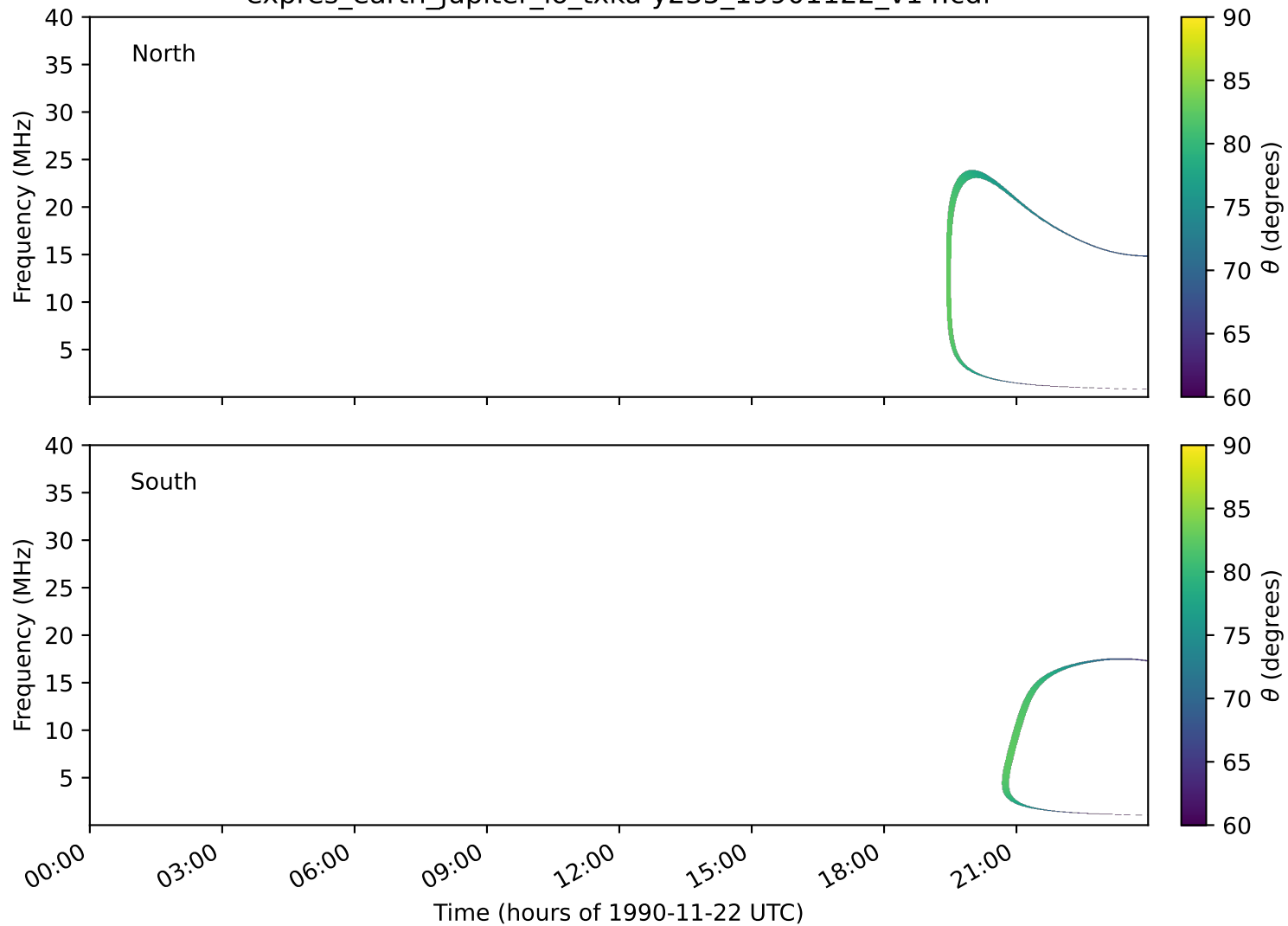
expres_earth_jupiter_io_txka-y235_19901122_v14.cdf
