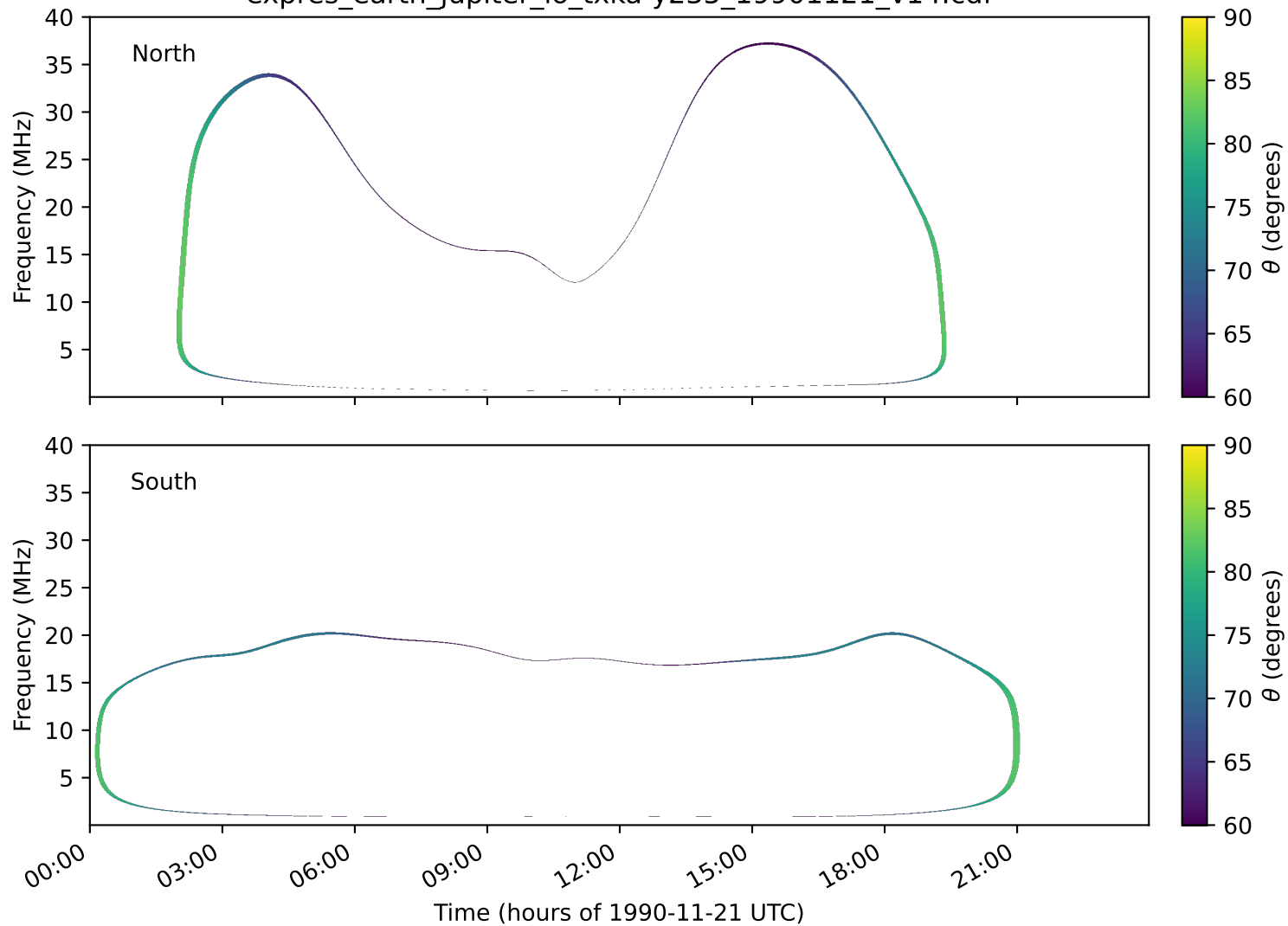
expres_earth_jupiter_io_txka-y235_19901121_v14.cdf
