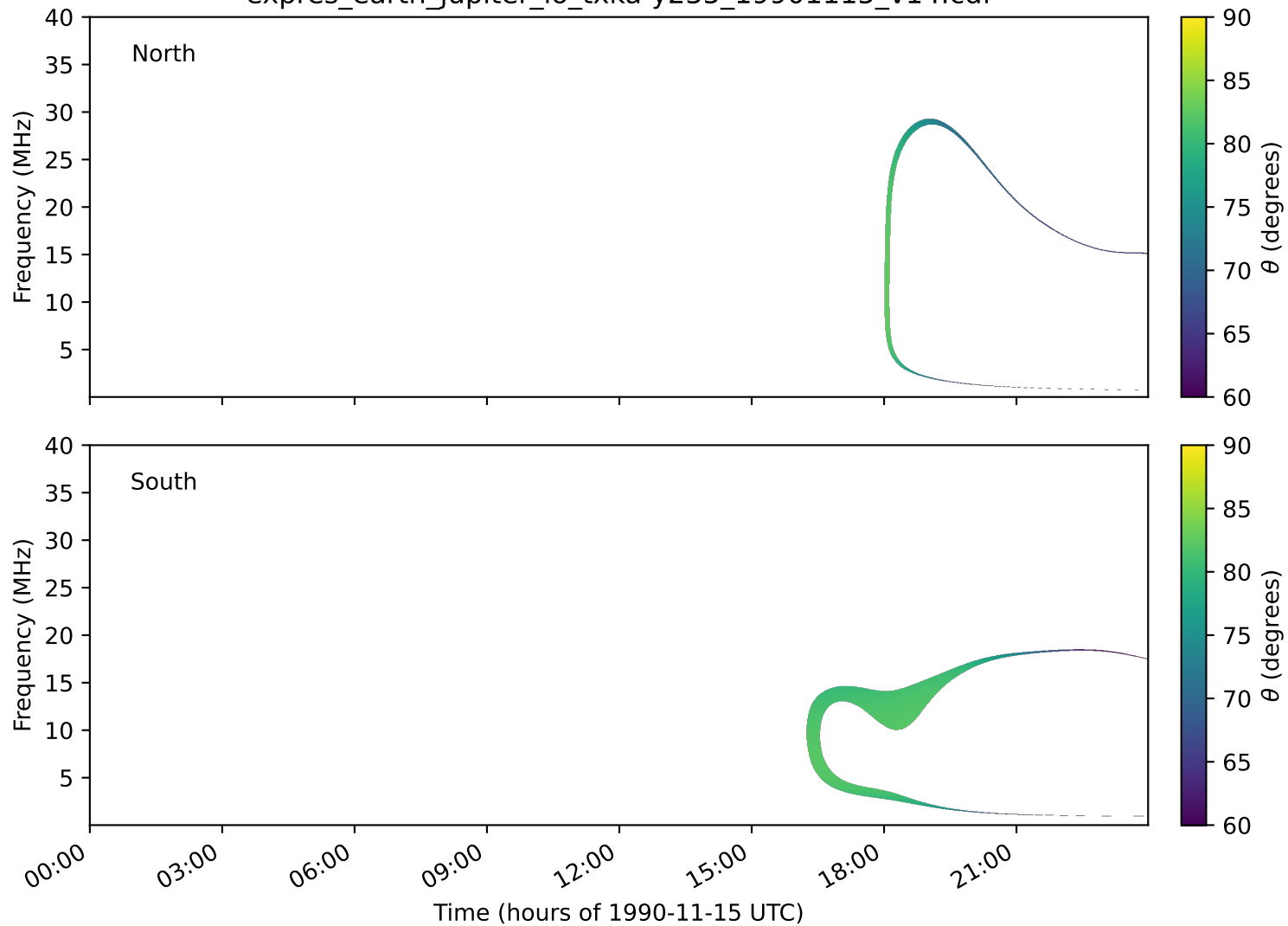
expres_earth_jupiter_io_txka-y235_19901115_v14.cdf
