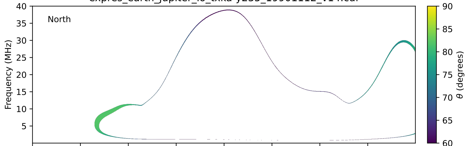
expres_earth_jupiter_io_txka-y235_19901112_v14.cdf
