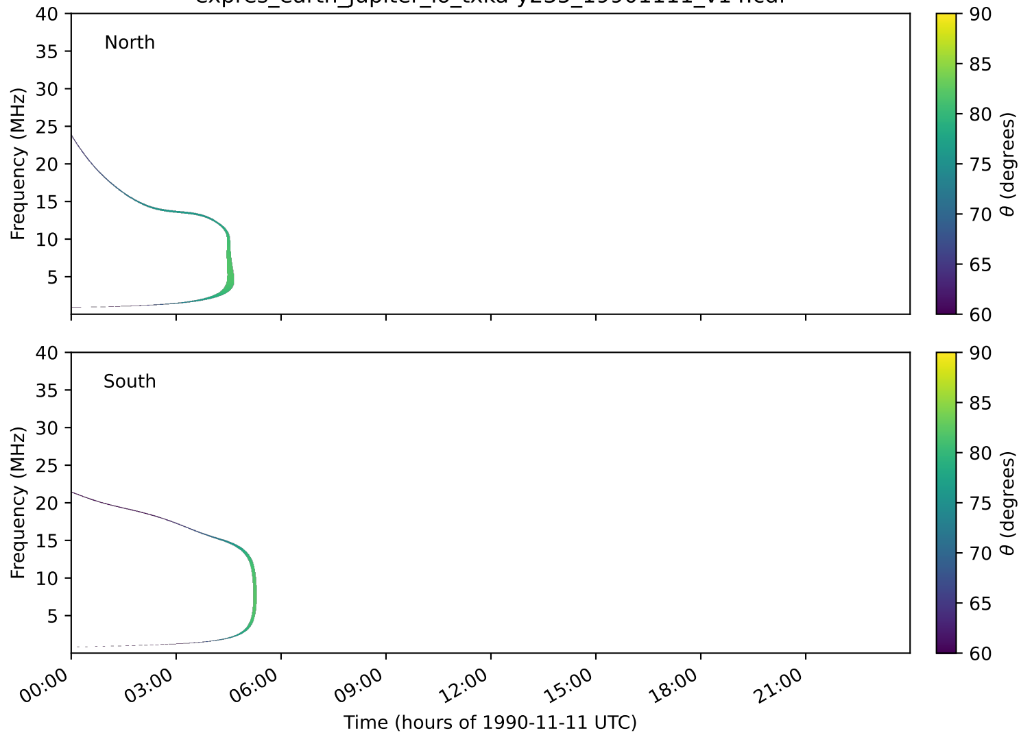
expres_earth_jupiter_io_txka-y235_19901111_v14.cdf
