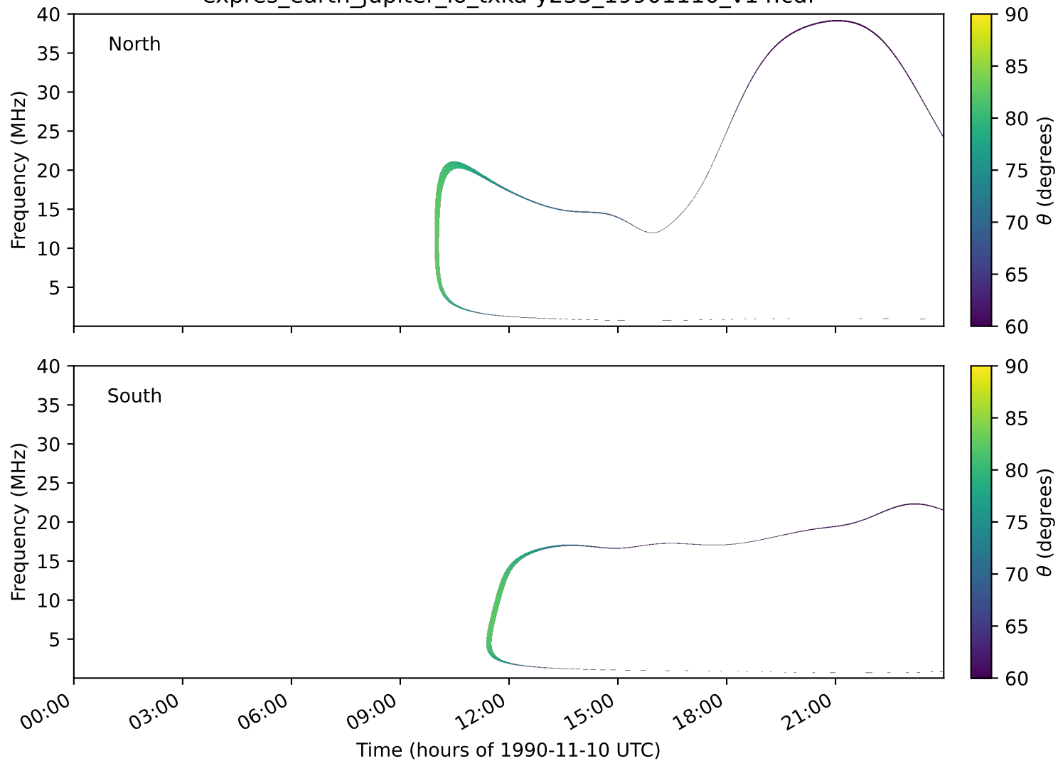
expres_earth_jupiter_io_txka-y235_19901110_v14.cdf
