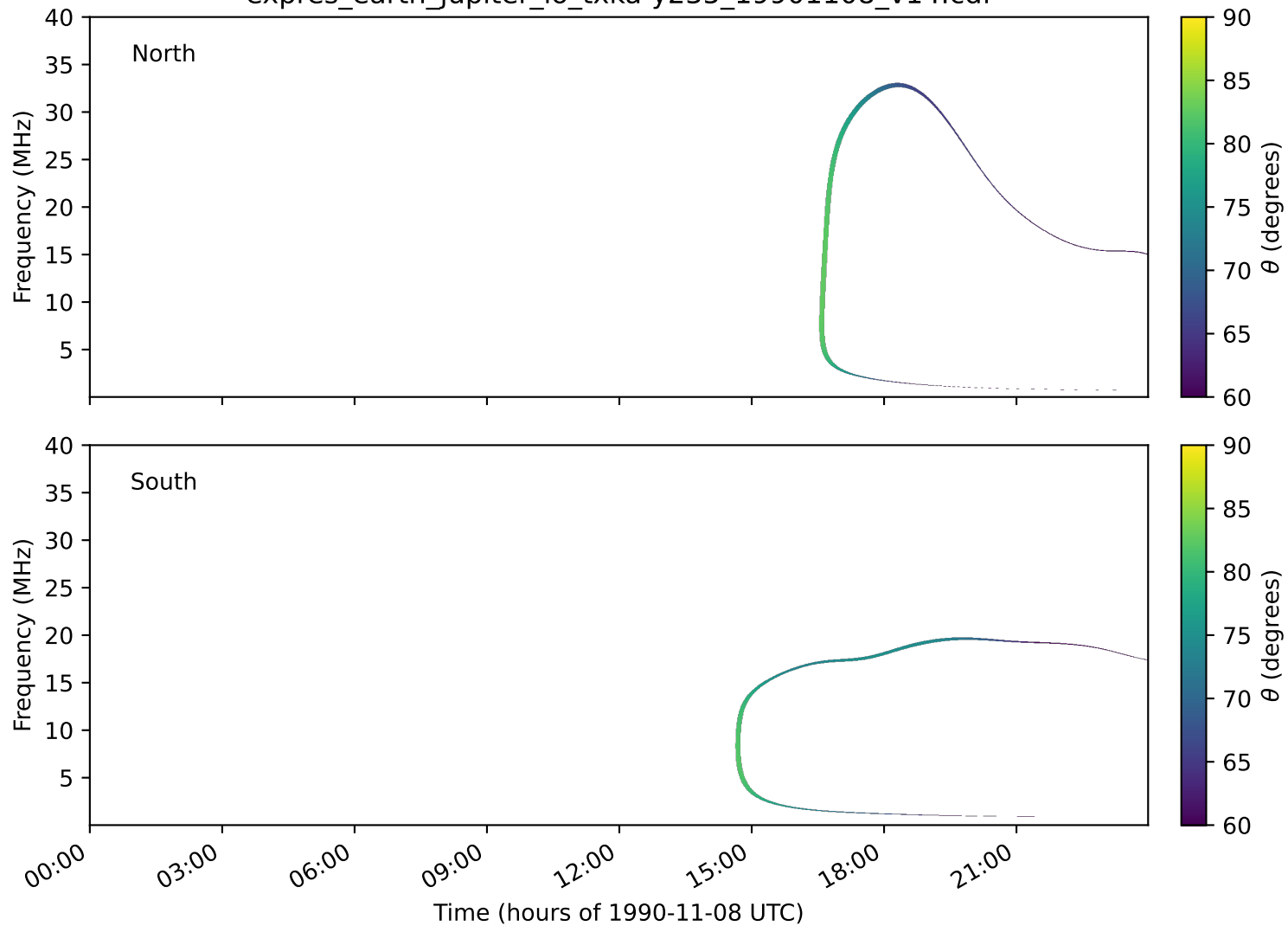
expres_earth_jupiter_io_txka-y235_19901108_v14.cdf
