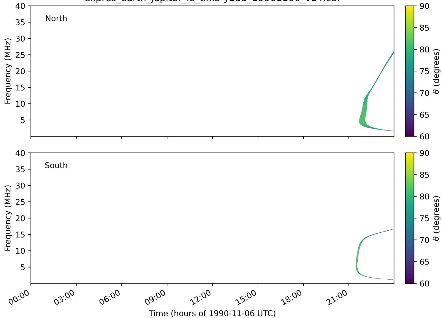
expres_earth_jupiter_io_txka-y235_19901106_v14.cdf
