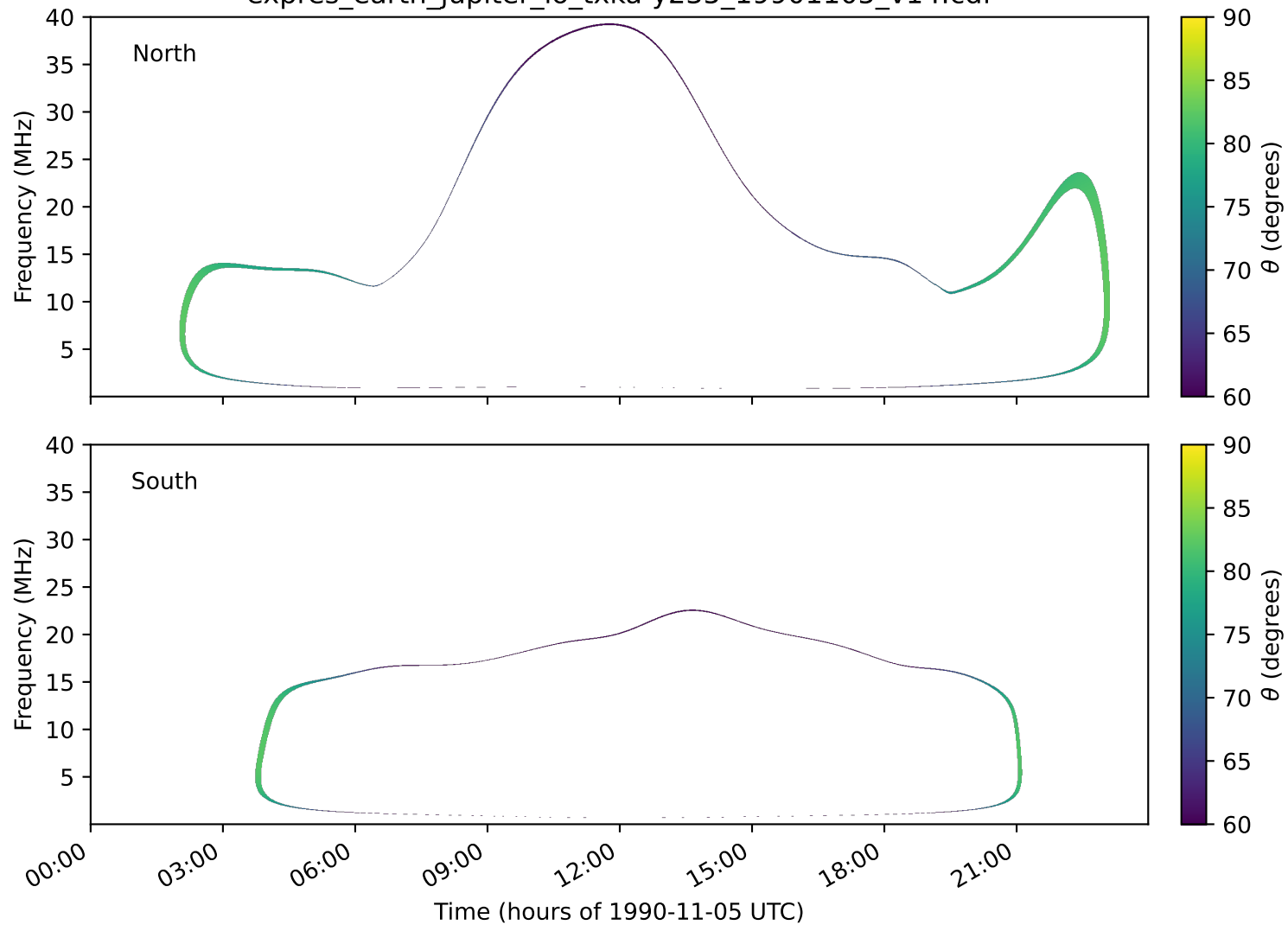
expres_earth_jupiter_io_txka-y235_19901105_v14.cdf
