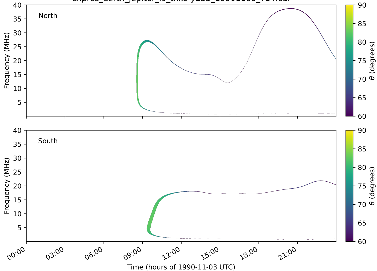
expres_earth_jupiter_io_txka-y235_19901103_v14.cdf
