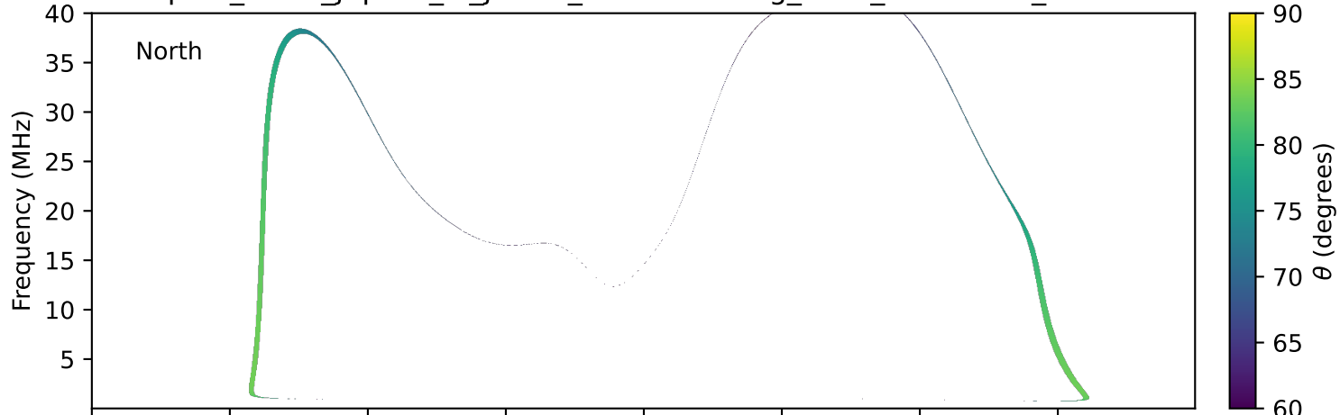
expres_earth_jupiter_io_jrm33_lossc-wid1deg_3kev_19901128_v11.cdf
