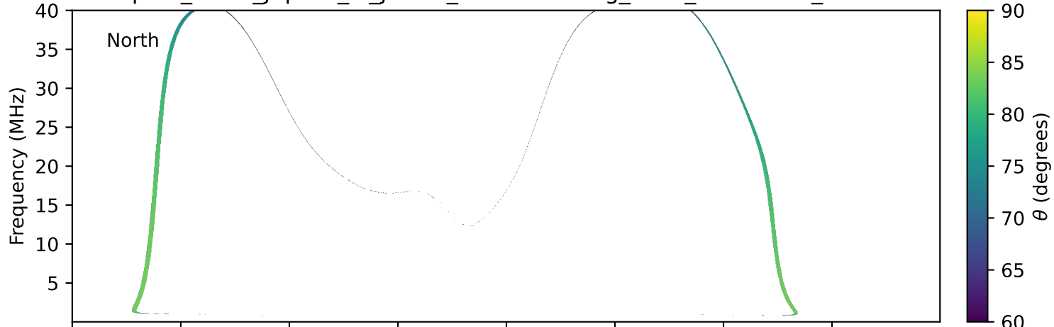
expres_earth_jupiter_io_jrm33_lossc-wid1deg_3kev_19901121_v11.cdf
