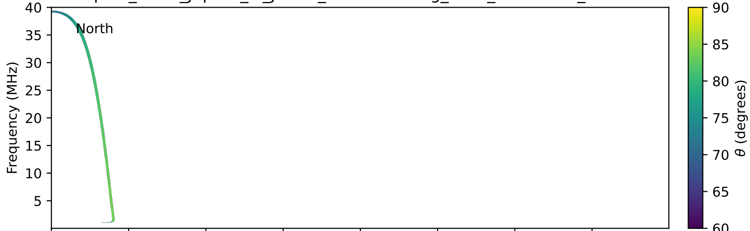
expres_earth_jupiter_io_jrm33_lossc-wid1deg_3kev_19901120_v11.cdf
