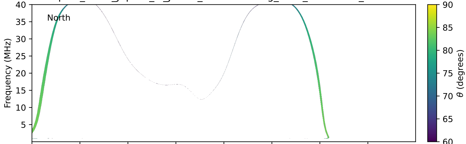
expres_earth_jupiter_io_jrm33_lossc-wid1deg_3kev_19901114_v11.cdf
