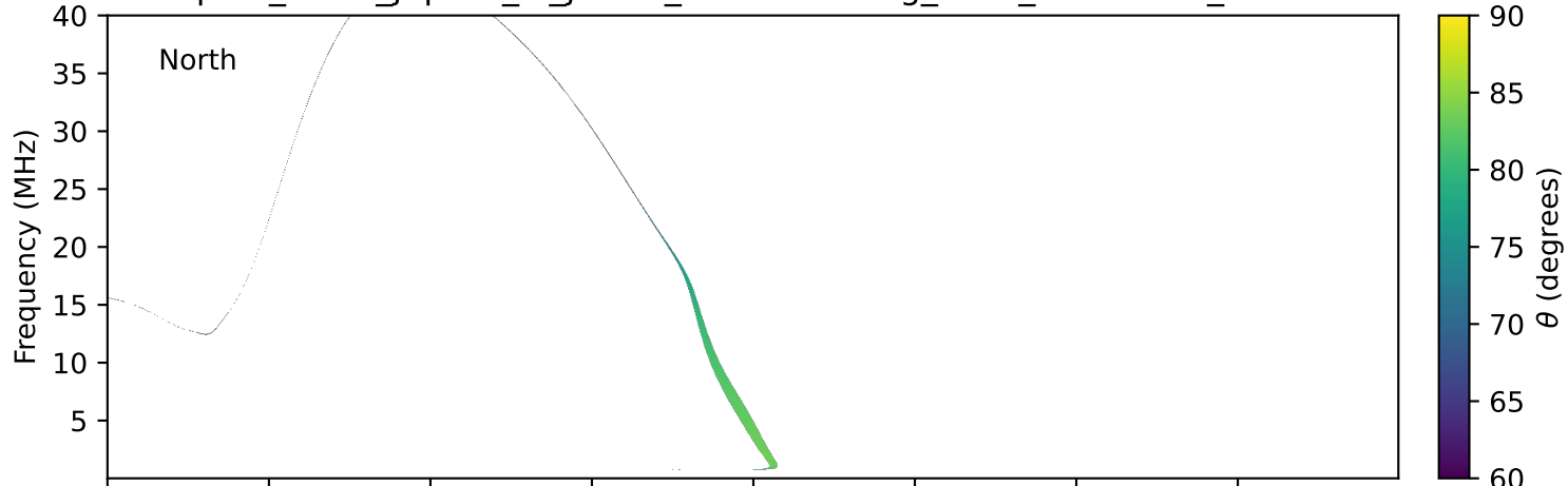
expres_earth_jupiter_io_jrm09_lossc-wid1deg_3kev_19901116_v11.cdf
