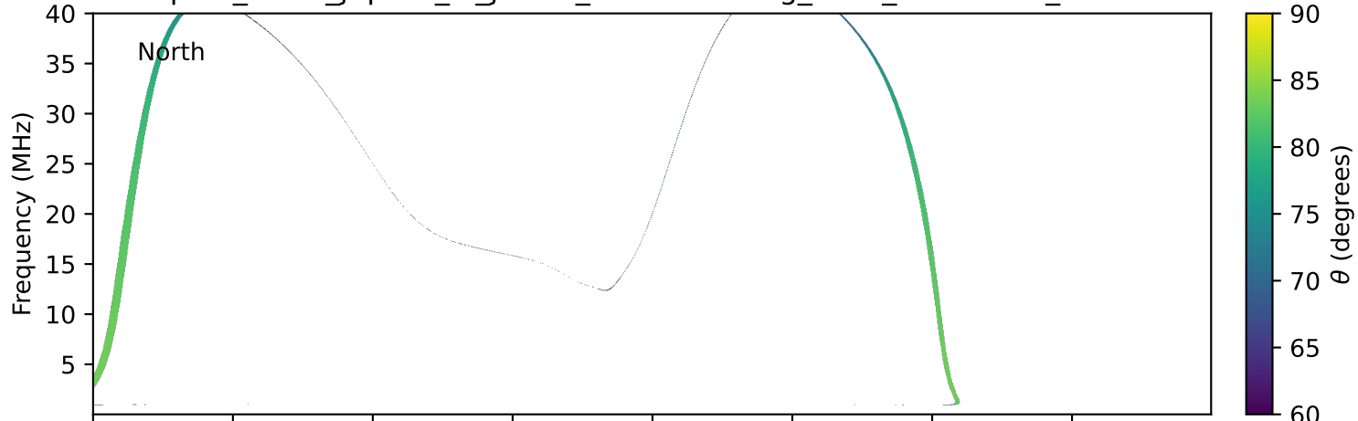
expres_earth_jupiter_io_jrm09_lossc-wid1deg_3kev_19901114_v11.cdf
