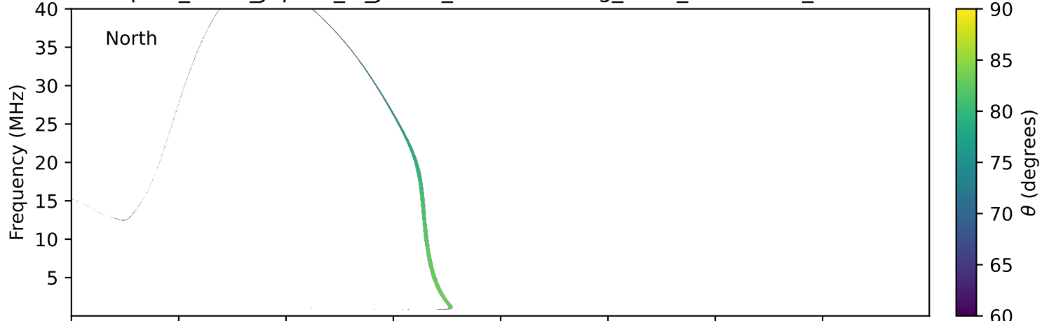
expres_earth_jupiter_io_jrm09_lossc-wid1deg_3kev_19901109_v11.cdf
