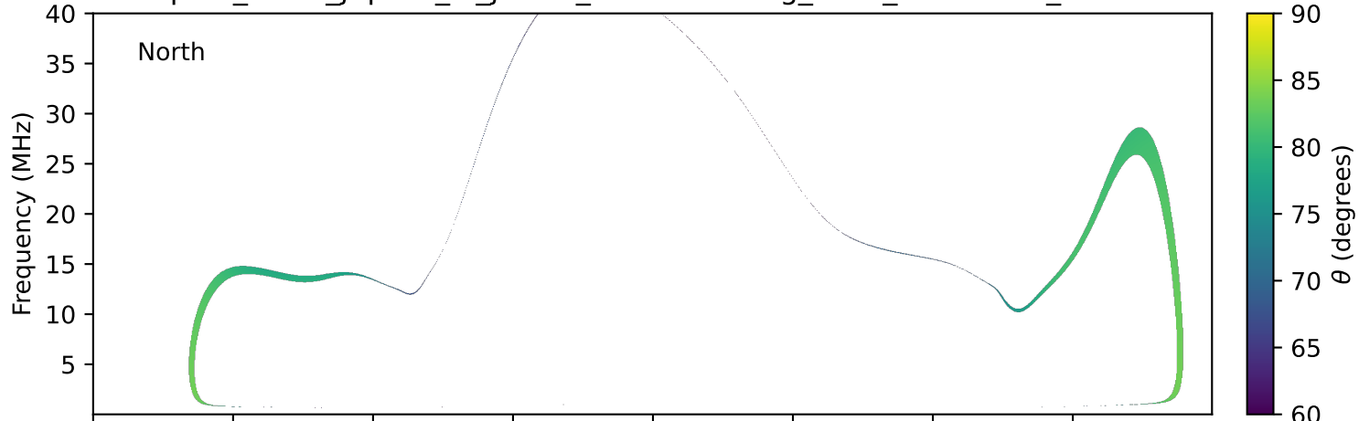
expres_earth_jupiter_io_jrm09_lossc-wid1deg_3kev_19901105_v11.cdf
