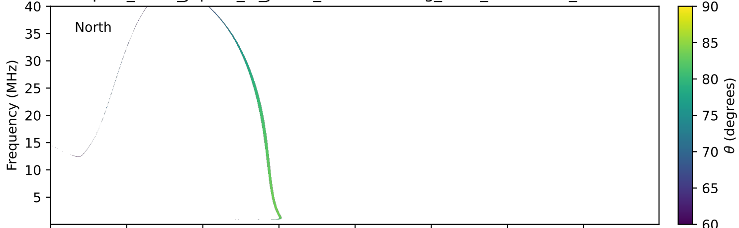
expres_earth_jupiter_io_jrm09_lossc-wid1deg_3kev_19901102_v11.cdf
