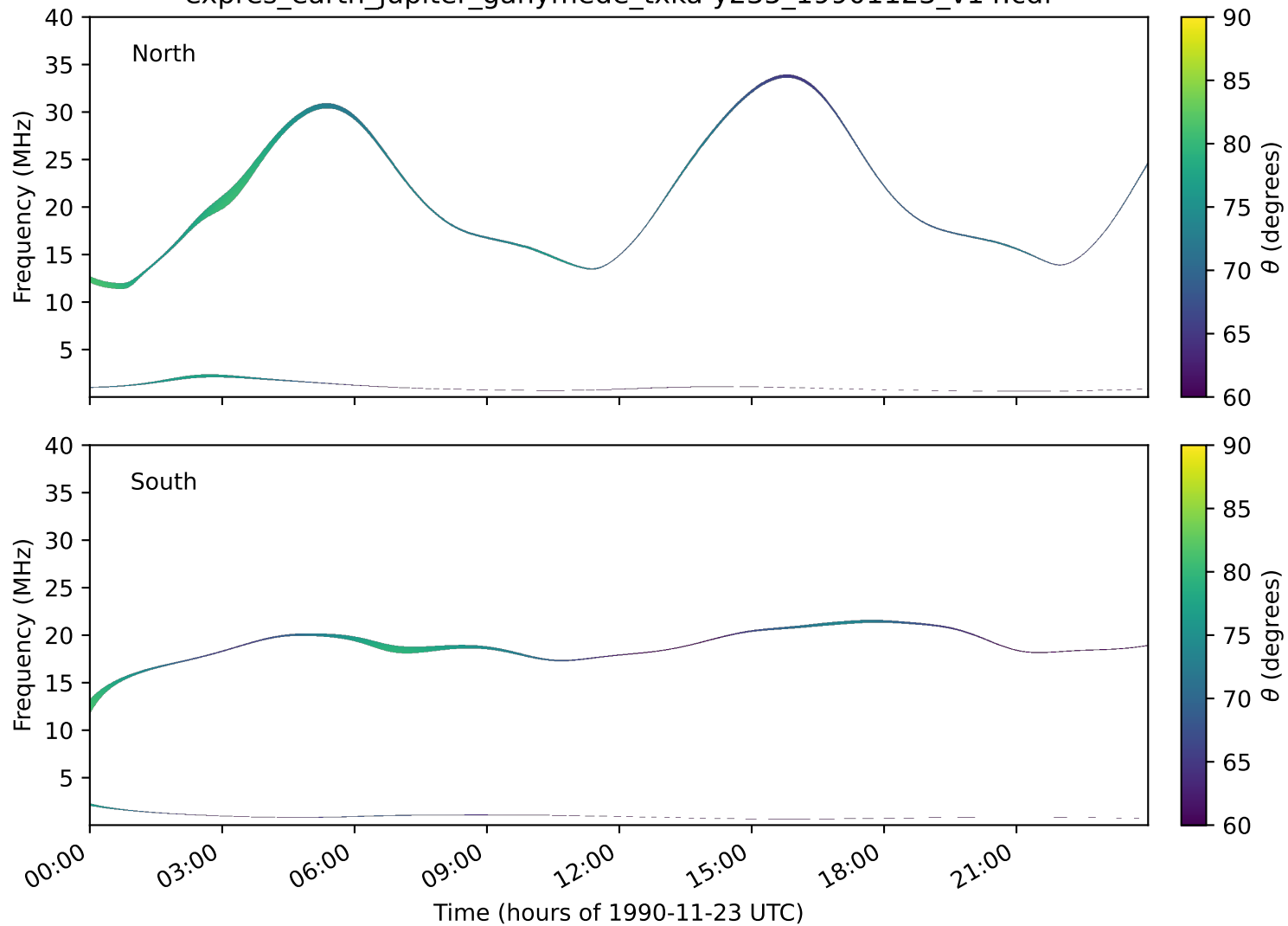
expres_earth_jupiter_ganymede_txka-y235_19901123_v14.cdf
