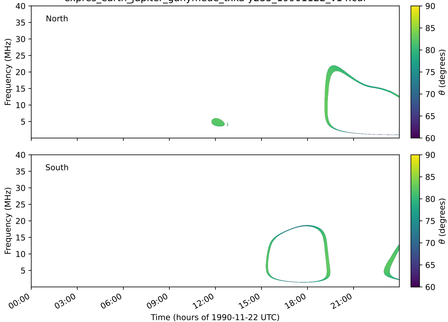
expres_earth_jupiter_ganymede_txka-y235_19901122_v14.cdf
