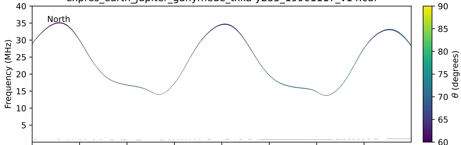
expres_earth_jupiter_ganymede_txka-y235_19901117_v14.cdf
