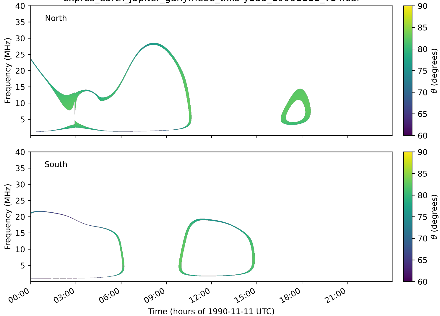
expres_earth_jupiter_ganymede_txka-y235_19901111_v14.cdf
