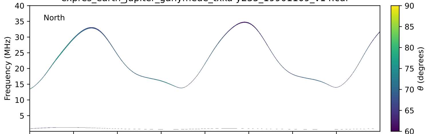
expres_earth_jupiter_ganymede_txka-y235_19901109_v14.cdf
