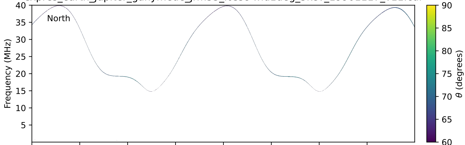
expres_earth_jupiter_ganymede_jrm33_lossc-wid1deg_3kev_19901117_v11.cdf
