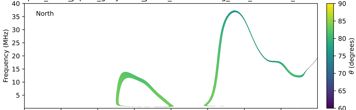
expres_earth_jupiter_ganymede_jrm33_lossc-wid1deg_3kev_19901101_v11.cdf
