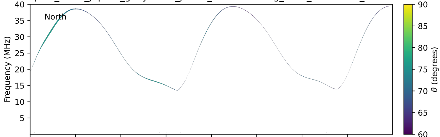
expres_earth_jupiter_ganymede_jrm09_lossc-wid1deg_3kev_19901102_v11.cdf
