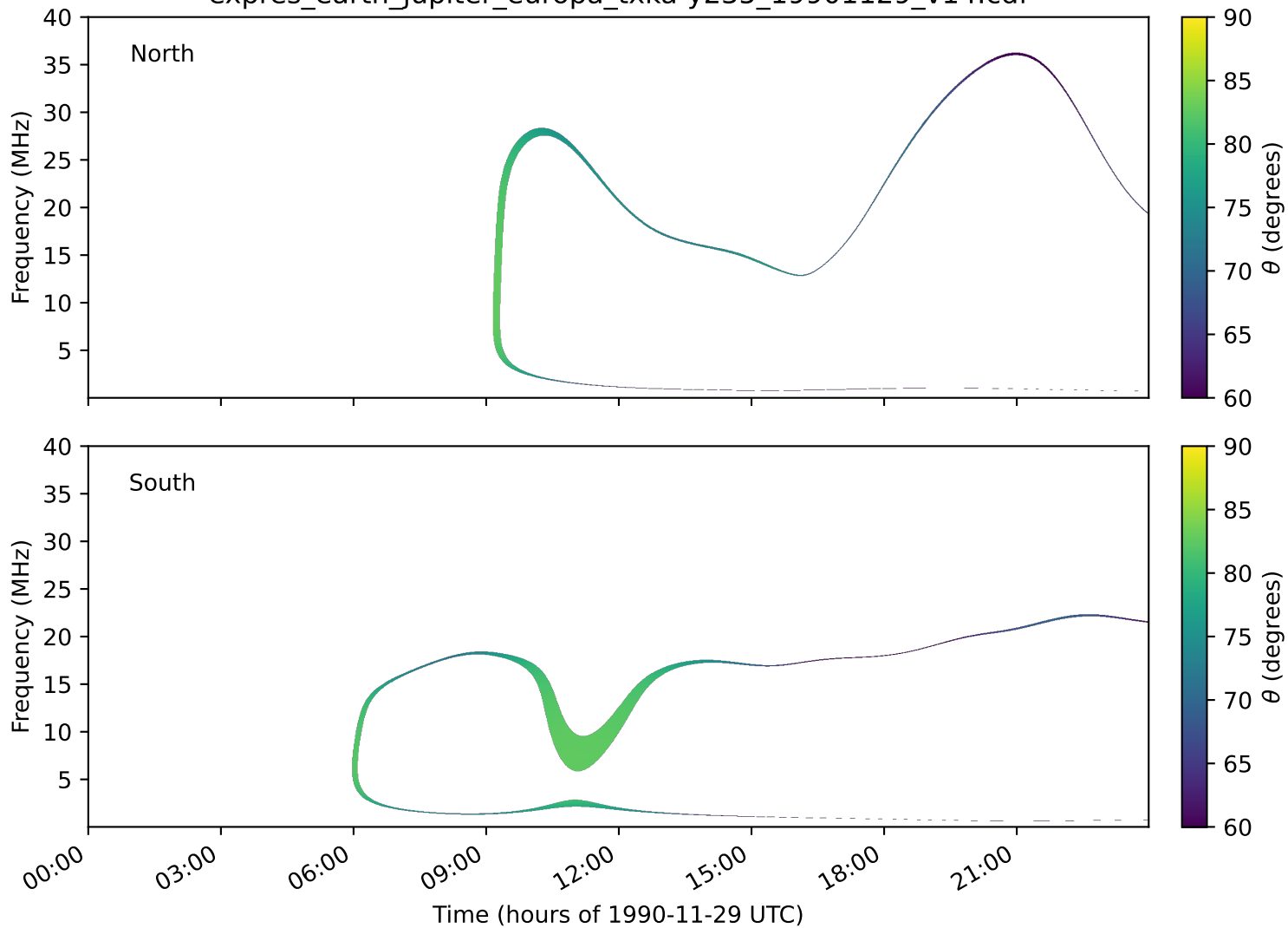
expres_earth_jupiter_europa_txka-y235_19901129_v14.cdf
