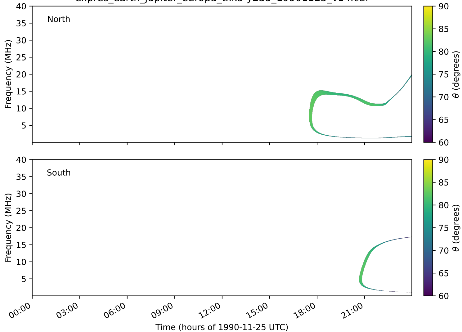
expres_earth_jupiter_europa_txka-y235_19901125_v14.cdf
