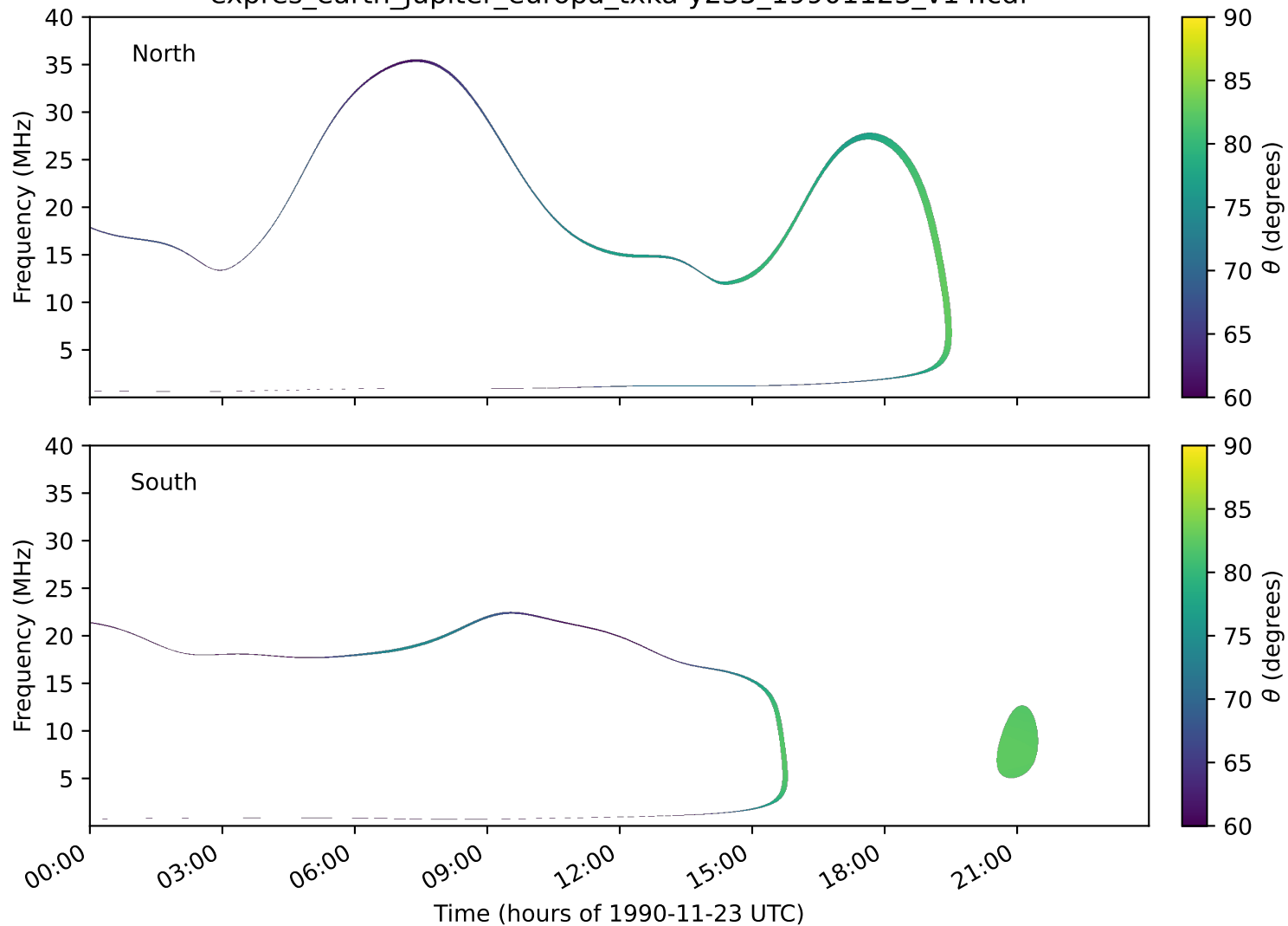
expres_earth_jupiter_europa_txka-y235_19901123_v14.cdf
