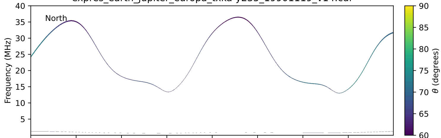
expres_earth_jupiter_europa_txka-y235_19901119_v14.cdf
