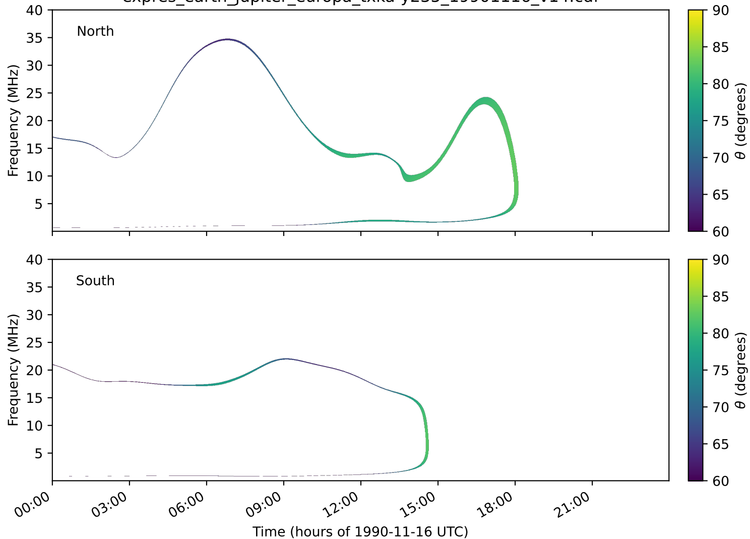
expres_earth_jupiter_europa_txka-y235_19901116_v14.cdf
