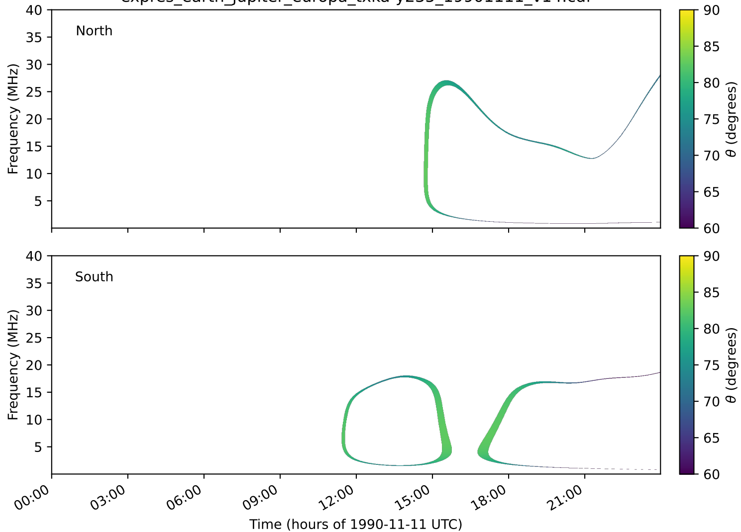
expres_earth_jupiter_europa_txka-y235_19901111_v14.cdf
