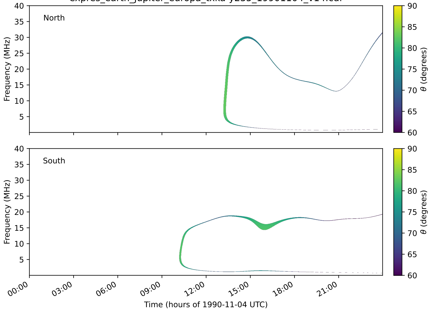
expres_earth_jupiter_europa_txka-y235_19901104_v14.cdf
