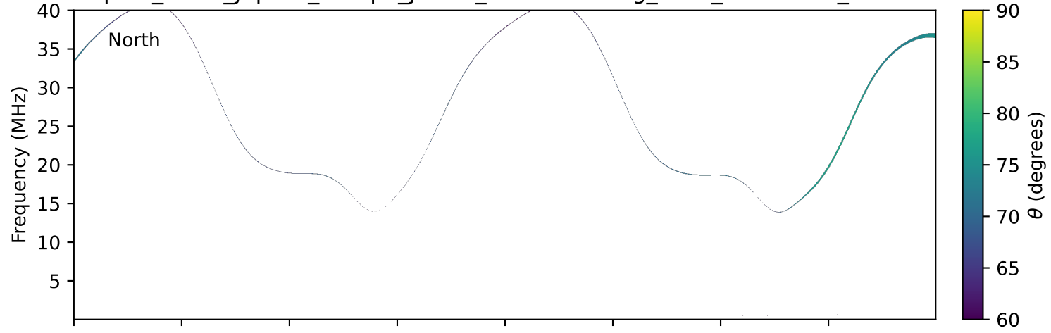
expres_earth_jupiter_europa_jrm33_lossc-wid1deg_3kev_19901112_v11.cdf
