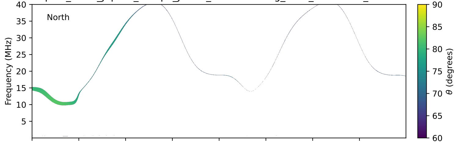
expres_earth_jupiter_europa_jrm33_lossc-wid1deg_3kev_19901101_v11.cdf
