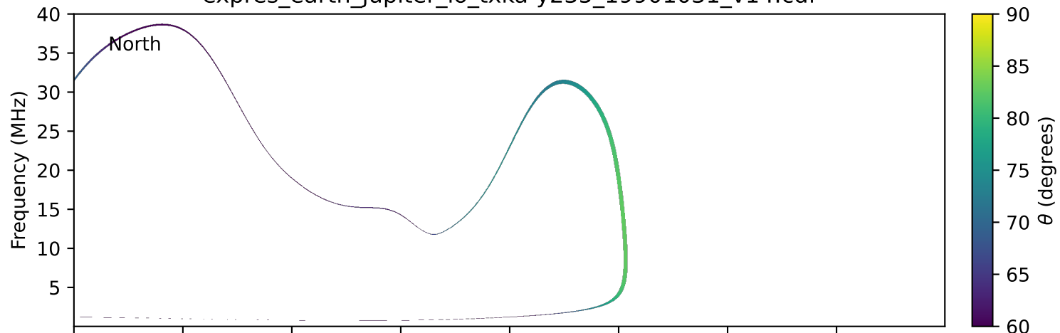
expres_earth_jupiter_io_txka-y235_19901031_v14.cdf
