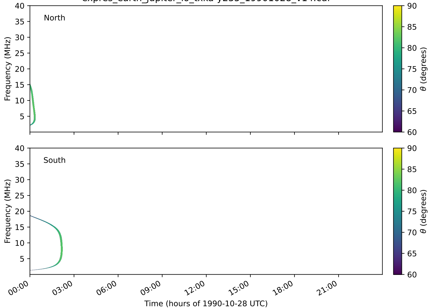
expres_earth_jupiter_io_txka-y235_19901028_v14.cdf
