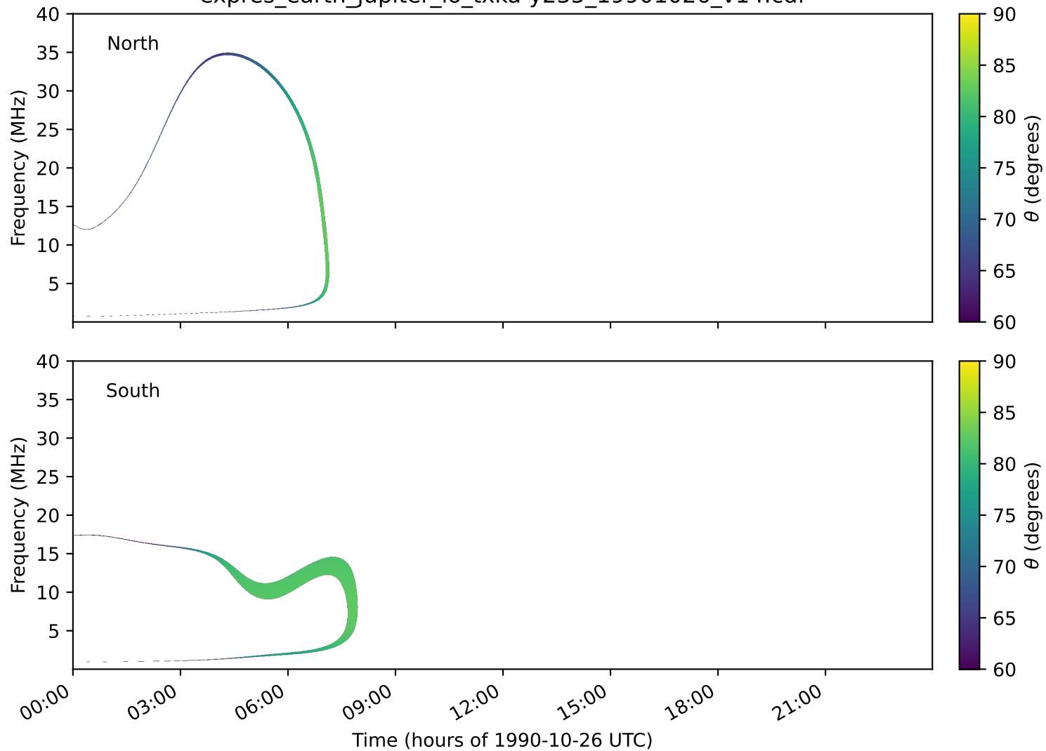
expres_earth_jupiter_io_txka-y235_19901026_v14.cdf
