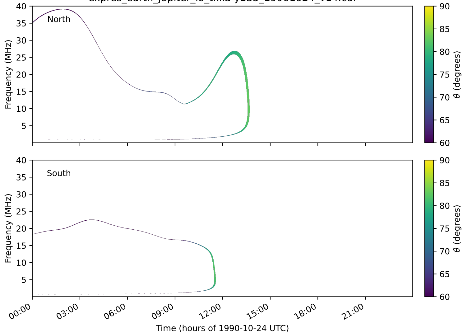
expres_earth_jupiter_io_txka-y235_19901024_v14.cdf
