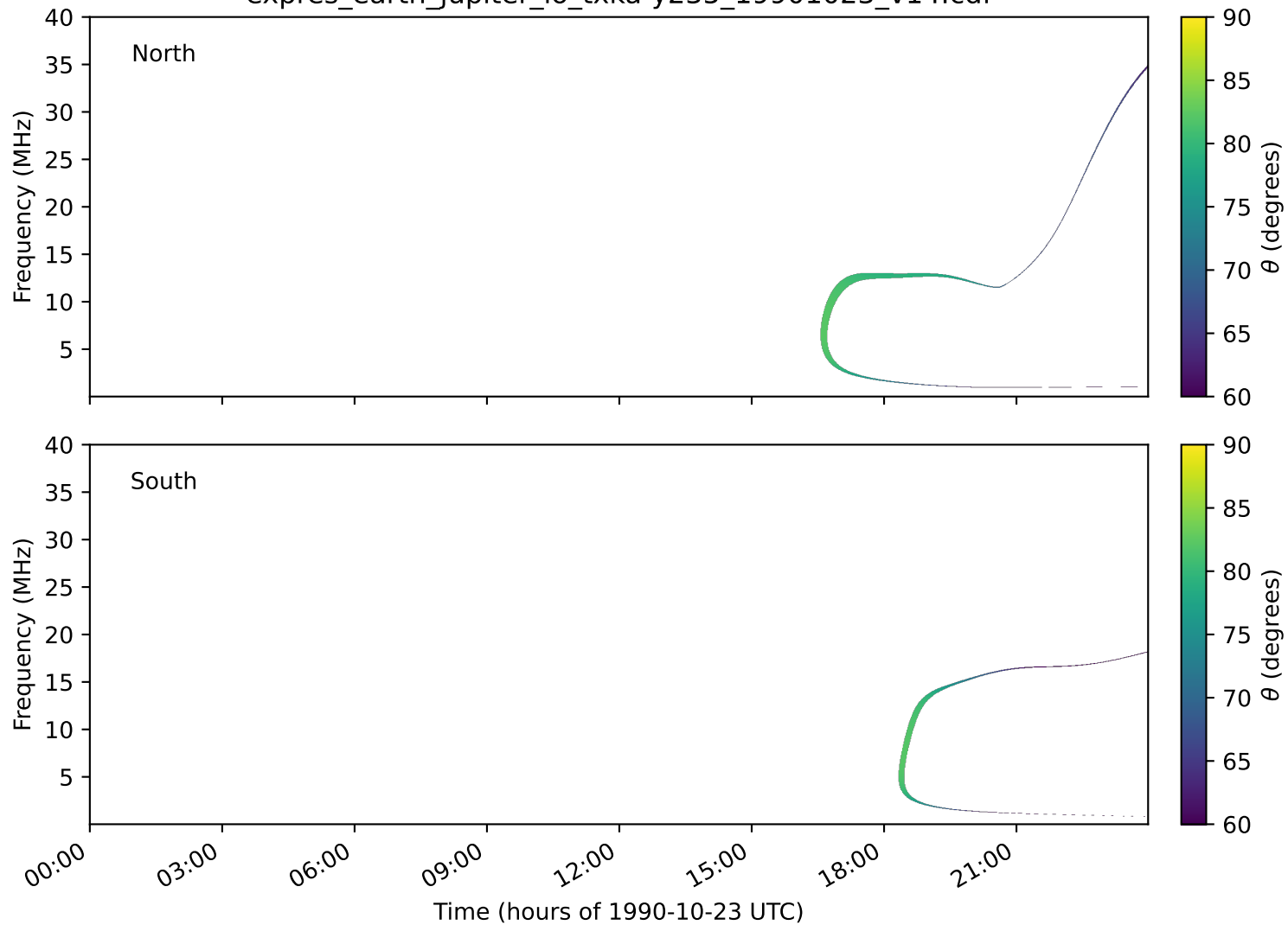
expres_earth_jupiter_io_txka-y235_19901023_v14.cdf
