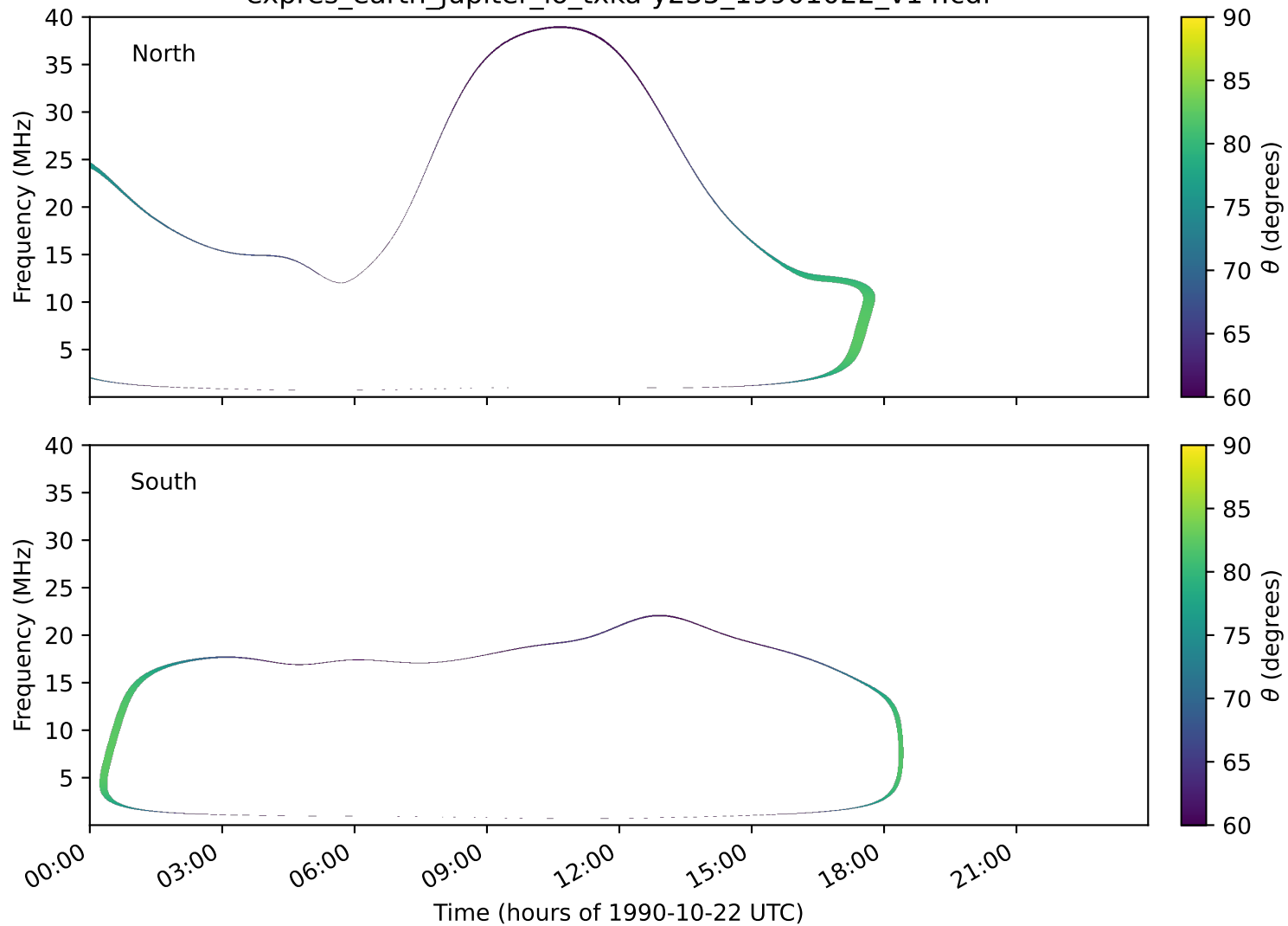
expres_earth_jupiter_io_txka-y235_19901022_v14.cdf
