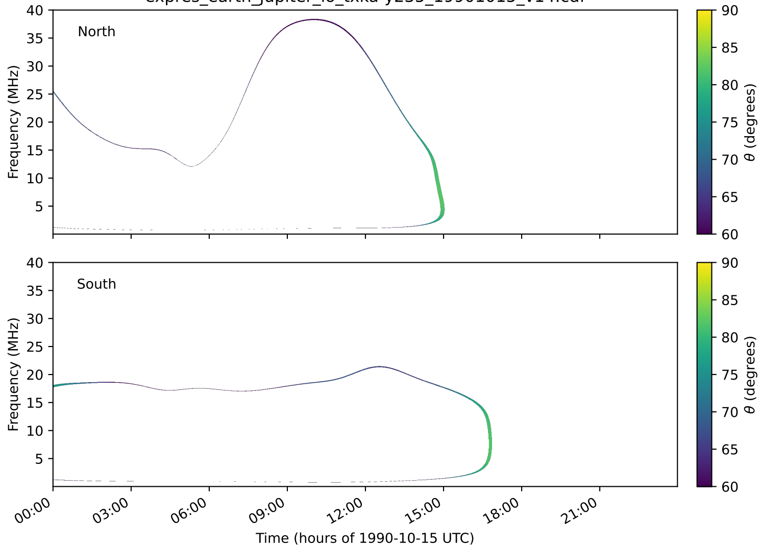
expres_earth_jupiter_io_txka-y235_19901015_v14.cdf
