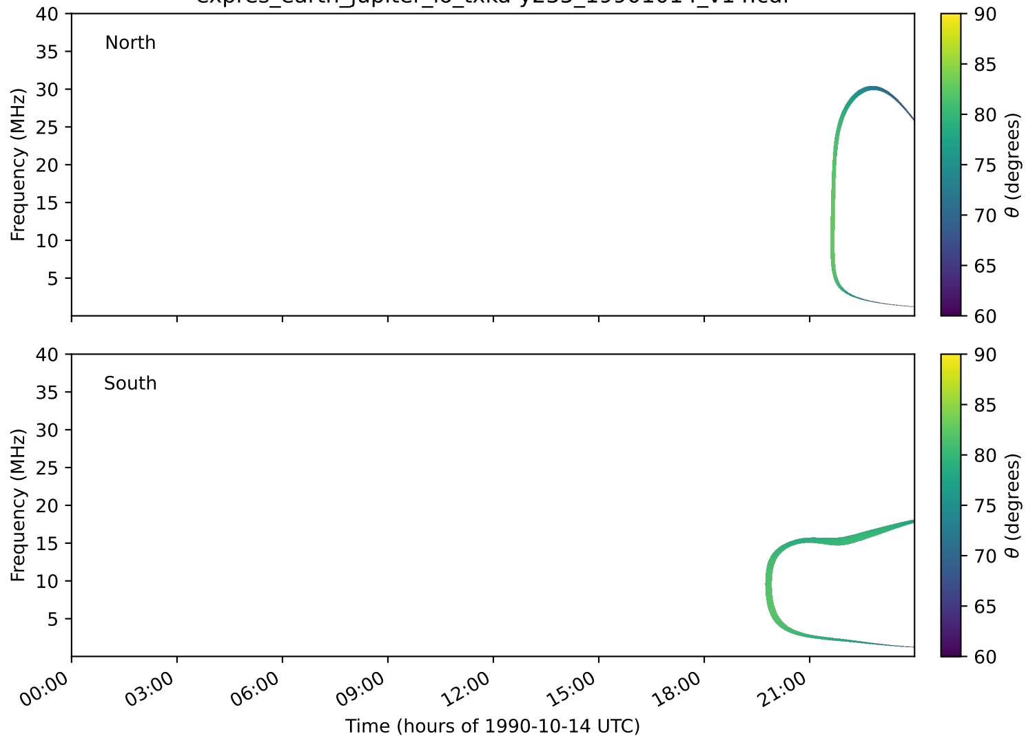
expres_earth_jupiter_io_txka-y235_19901014_v14.cdf
