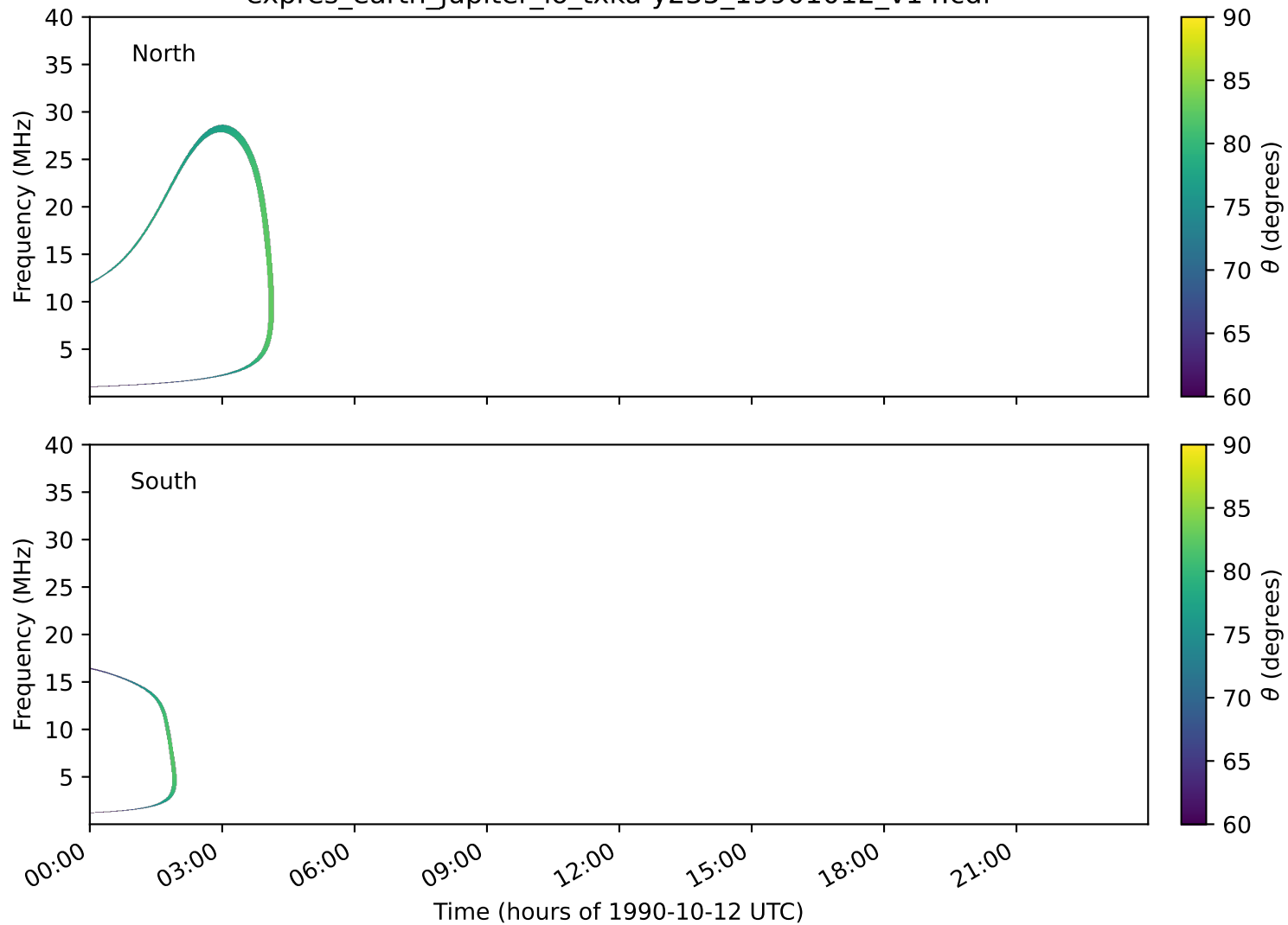
expres_earth_jupiter_io_txka-y235_19901012_v14.cdf
