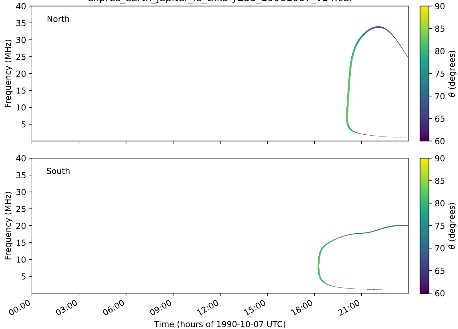
expres_earth_jupiter_io_txka-y235_19901007_v14.cdf
