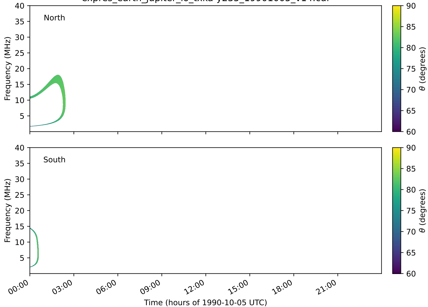
expres_earth_jupiter_io_txka-y235_19901005_v14.cdf
