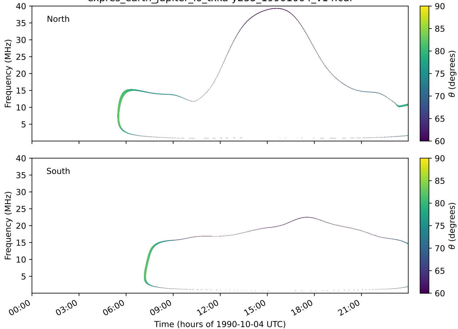
expres_earth_jupiter_io_txka-y235_19901004_v14.cdf
