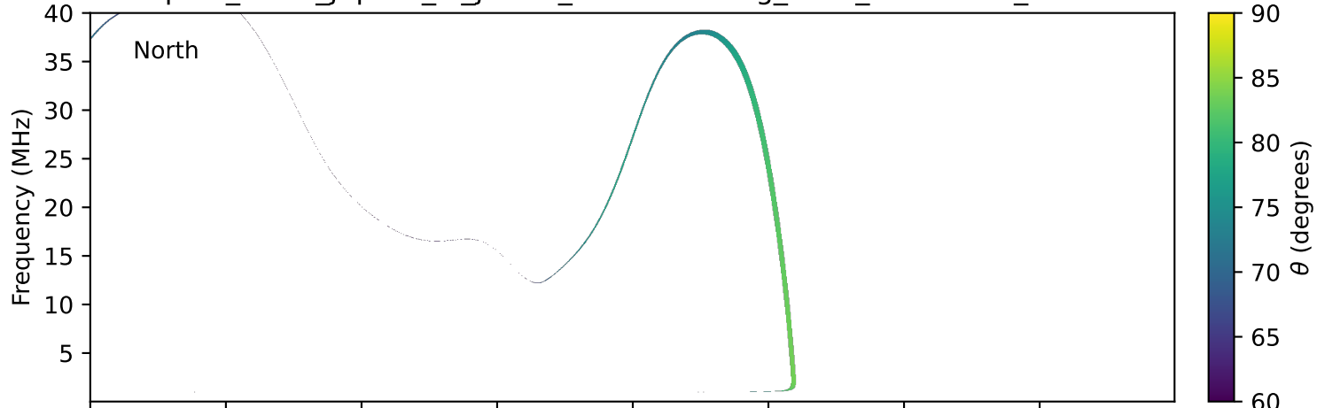
expres_earth_jupiter_io_jrm33_lossc-wid1deg_3kev_19901031_v11.cdf
