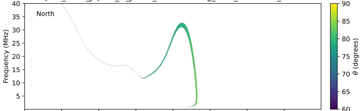
expres_earth_jupiter_io_jrm33_lossc-wid1deg_3kev_19901024_v11.cdf
